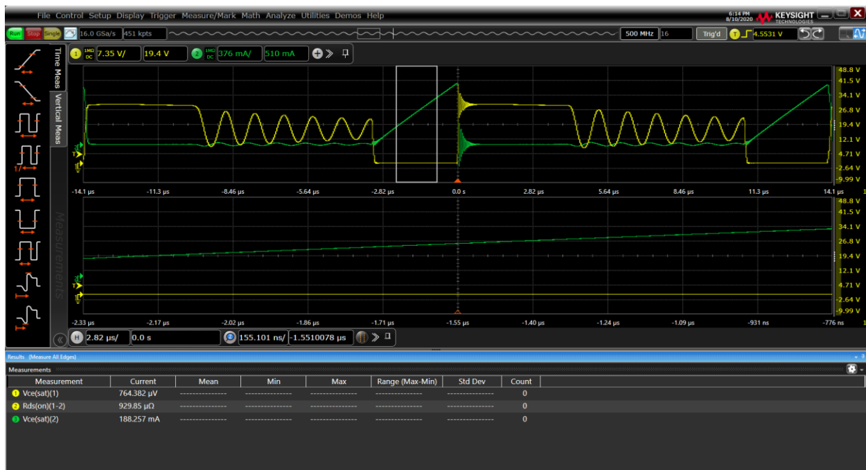
Figure 12. Measuring R_{ds(on)}
