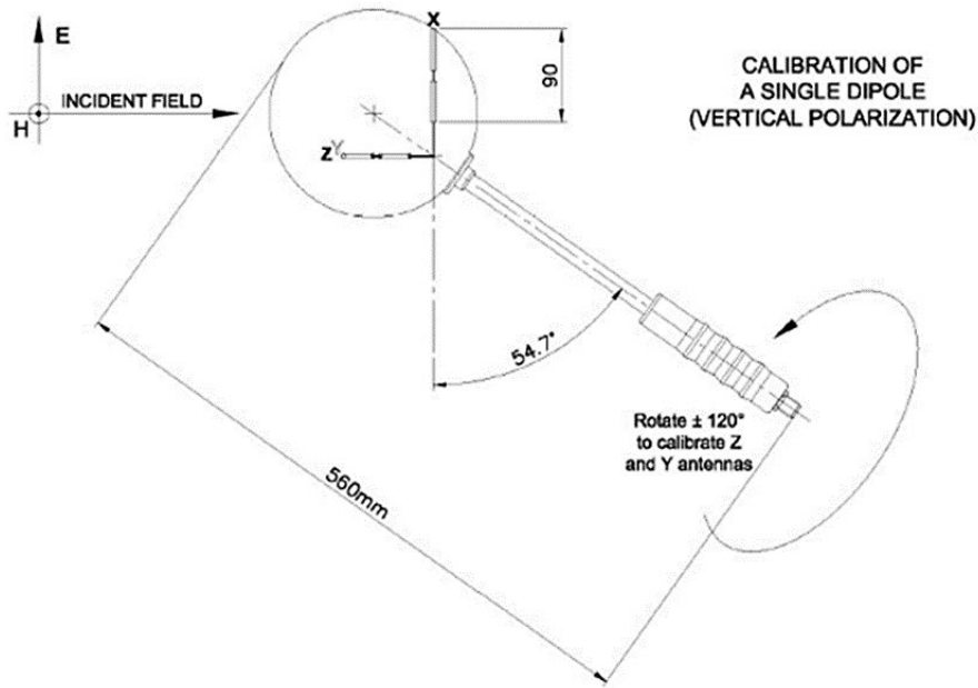
Figure 2. Calibration position and procedure for the 85572A-006 antenna
