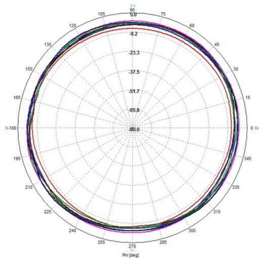
Figure 1. Isotropic radiation patterns for vertical and horizontal orientations
