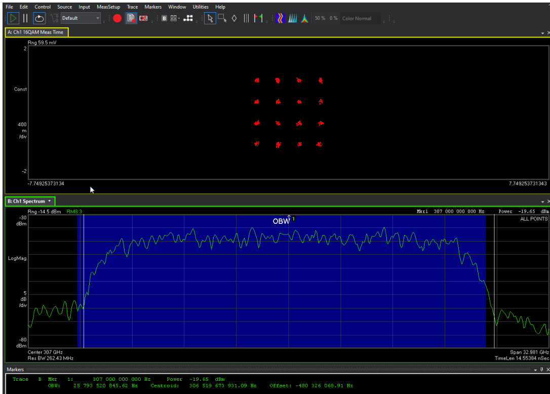
Figure 3. Conducted Measurement Results at 307 GHz for the 25.92 GHz Bandwidth Test Case
