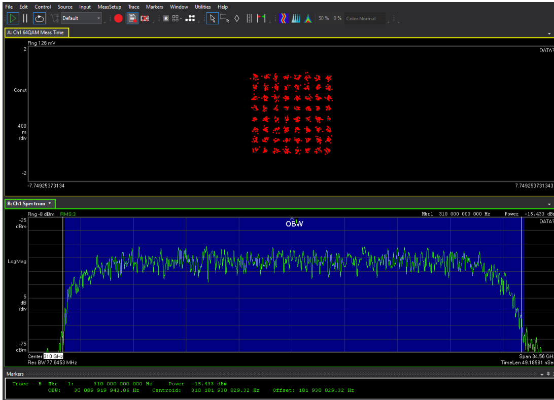
Figure 5. Over-the-air (OTA) Measurement Results at 310 GHz for the 30 GHz Bandwidth Test Case
